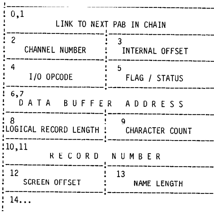
FIGURE C.5.1 Modified PAB Layout
