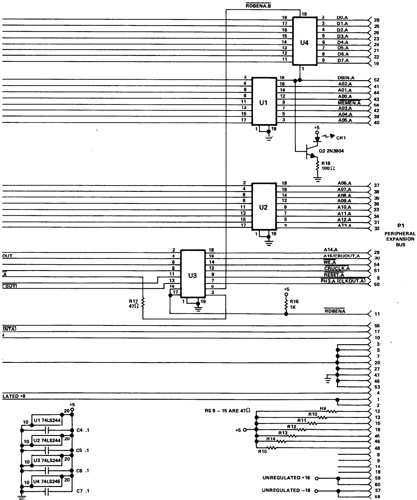
FLEX CABLE SCHEMATIC DIAGRAM (PERIPHERAL EXPANSION UNIT END OF CAE)
