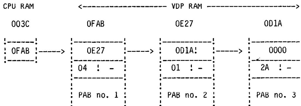
FIGURE C.5.2 BASIC Link Structure
