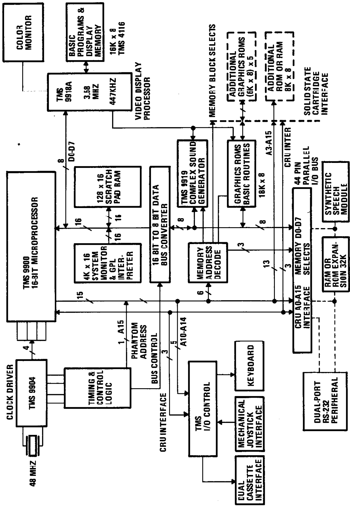
FIGURE A. T1-99/4A SYSTEM BLOCK DIAGRAM
