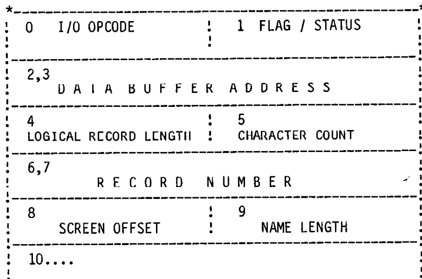
Figure C.3.1.1 PAB Layout
